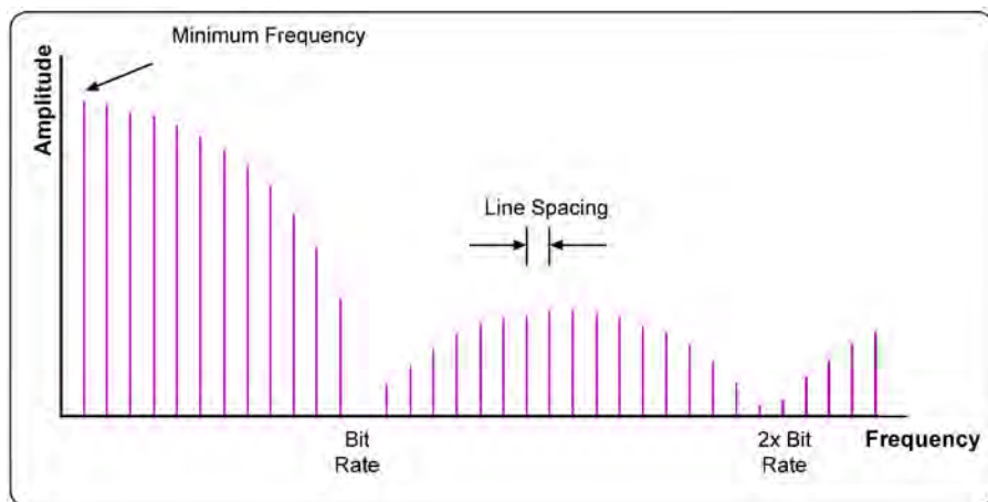
Figure 1. Reminder of an NRZ spectrum, with nulls at multiples of the bit rate, and \sin(x)/x envelope. The minimum frequency and line spacing are both given by the formula in the text, with examples in Table 1.
