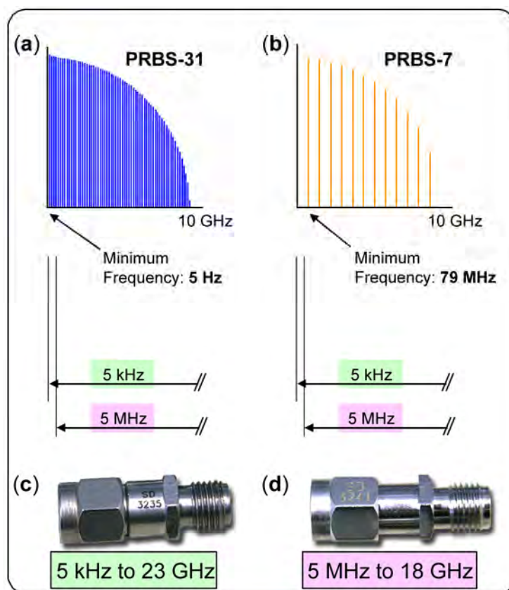
Figure 2. The minimum frequency in the longest common test pattern, PRBS-31 (a) is shown alongside one of the commonest short patterns, PRBS-7 (b). The minimum frequencies of two different models of d.c. blocks (c) and (d) are also shown.
