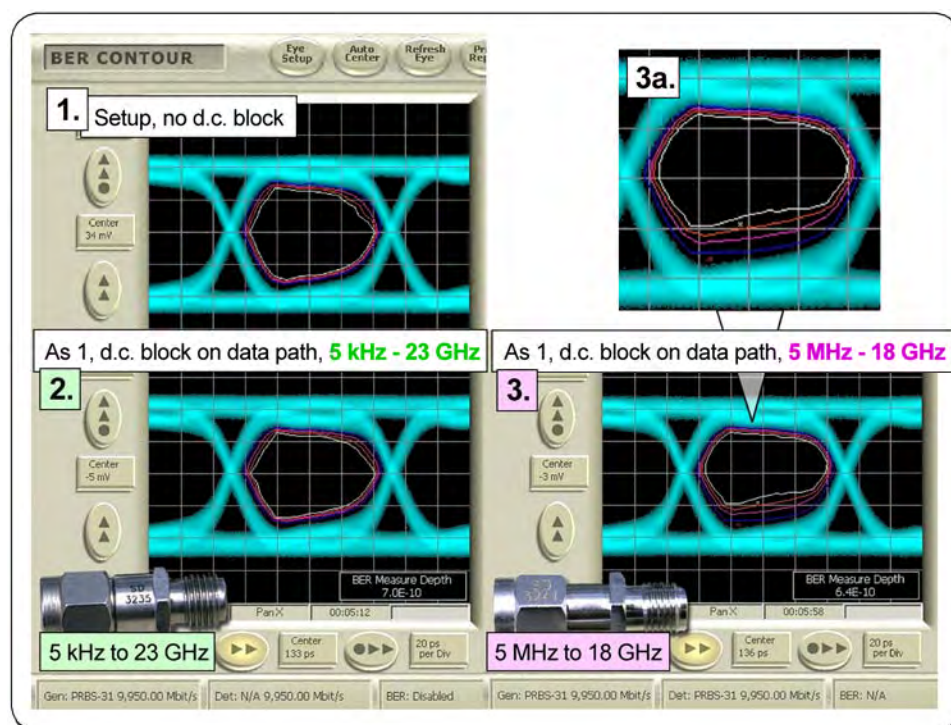
Figure 3. Passing 9.95 Gb/s data using a PRBS-31 pattern. (1) shows the signal after passing through the measurement setup but d.c. coupled; (2) has the better of the two d.c. blocks in place, (3) has a 5 MHz lower frequency cutoff and shows significant eye degradation.
